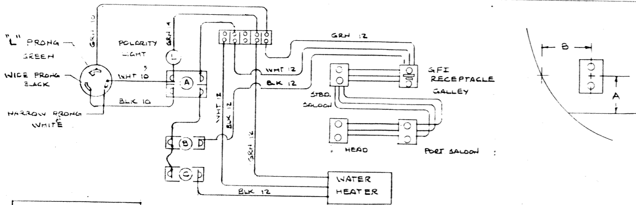
120 VAC SCHEMATIC
